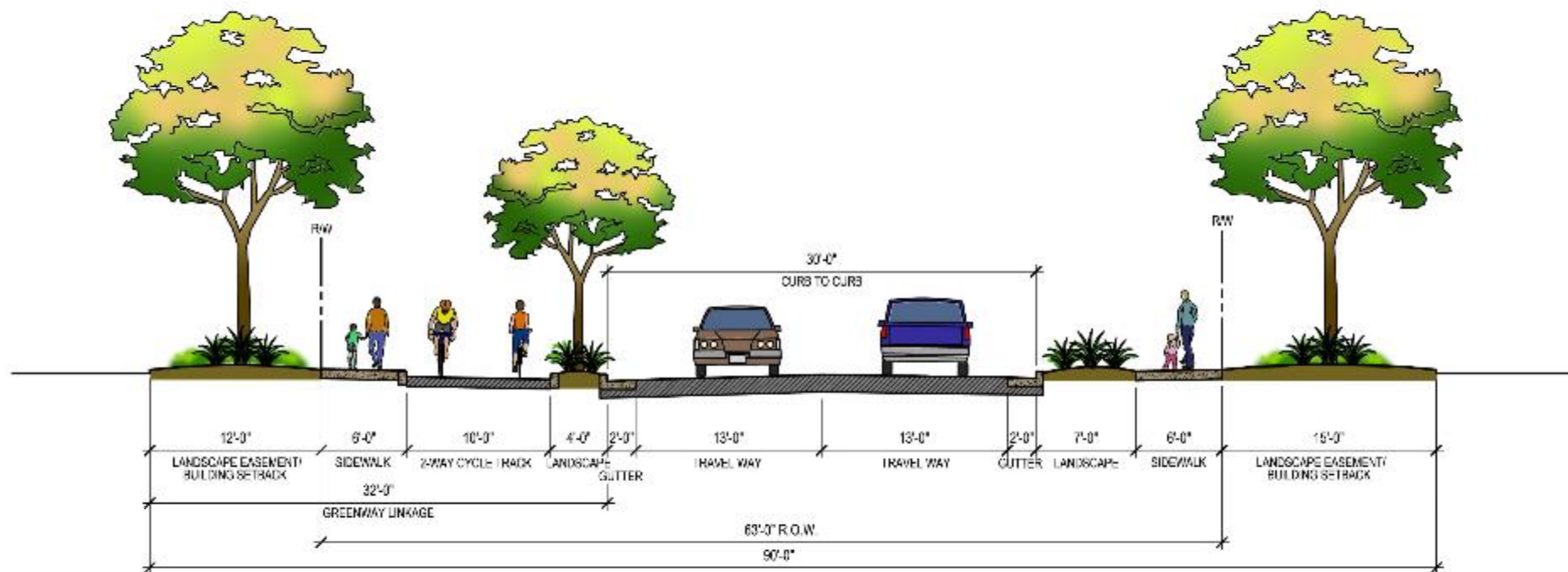
CYCLE TRACK AND SIDEWALK (63' ROW) - INCREMENT 1, OPTION 2 NO PARKING
